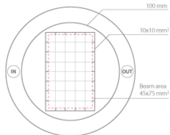
MIRROR BACK VIEW
