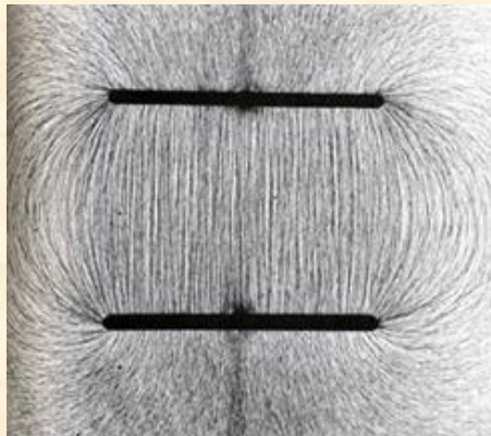
Electrons sources
