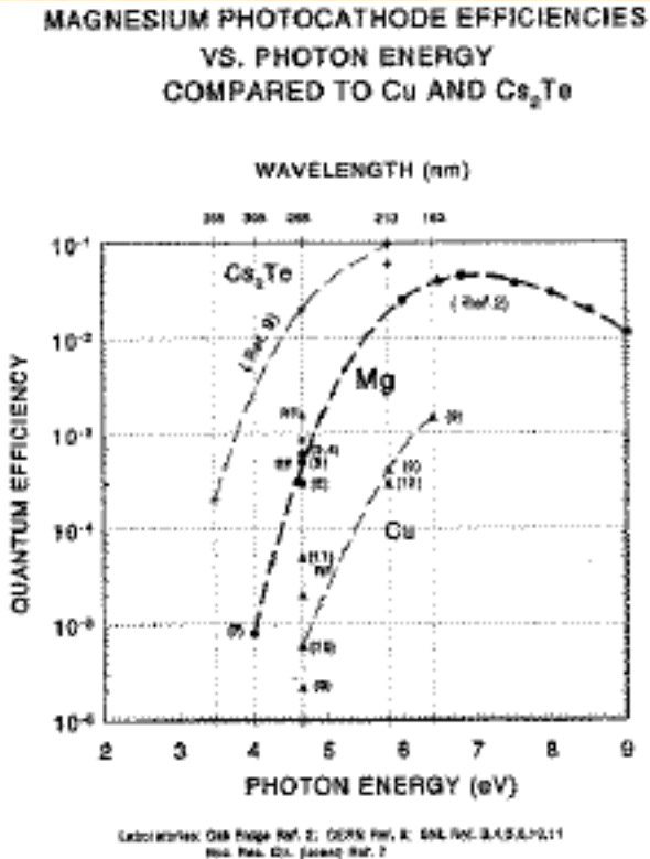
Figure 2: QE data for Cs 2 Te, Mg, and Cu photocathodes versus wavelength [0].
